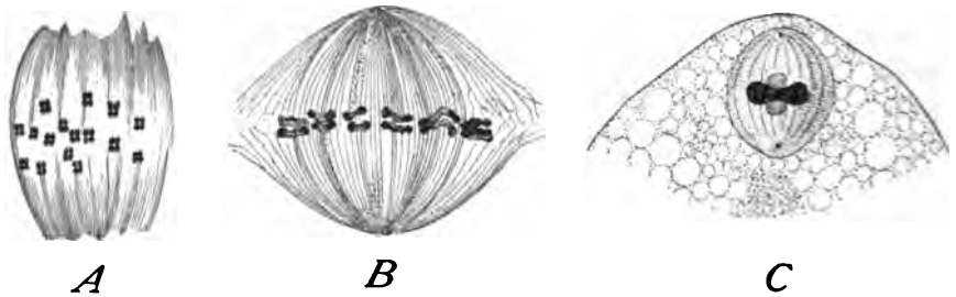
Fig. 137. — Types of maturation-spindles in the female.
